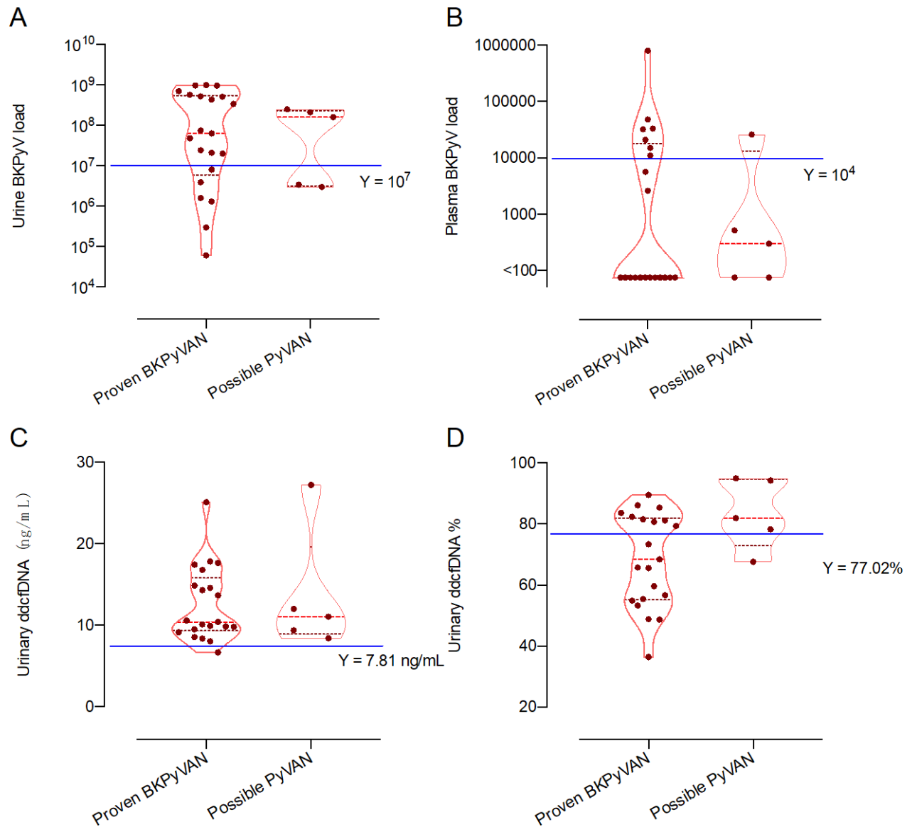
Fig. S3 Comparisons of urine and plasma BKPyV DNA loads and urine ddcfDNA levels in BKPyVAN diagnosis. Urine (A) and plasma (B) BKPyV DNA load; urinary ddcfDNA concentrations (C) and fractions (D). Blue solid line represents the cut of value.
