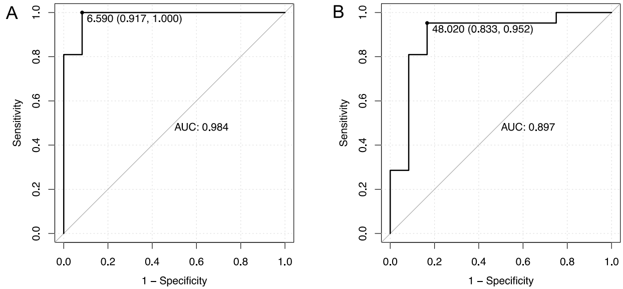
Fig. S1 Diagnostic performance of the concentration and fraction of ddcfDNA. ROC curve of ddcfDNA concentration (A) and fraction (B) in discriminating BKPyVAN and protocol biopsy.
