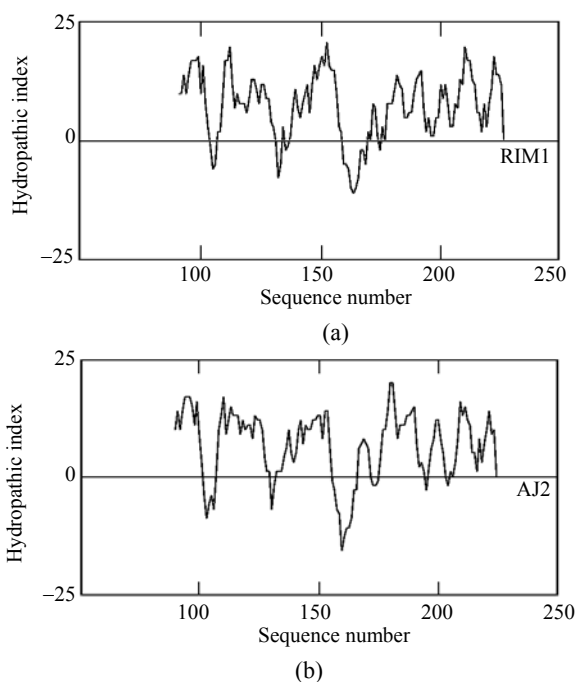
Fig.3 Hydropathic profile from amino acid residue 91 to 223 of Hbt. salinarium R1M1 BR (a) and AJ2 BR (b). The profile was calculated according to Kyte and Doolittle (1982). All plots utilize a span setting of 9
