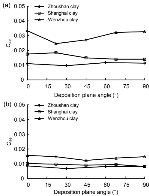
Fig. 11 Relationship between C_{ae} and deposition plane angle for three clays: (a) maximum C_{ae} ; (b) C_{ae} corresponding to a vertical stress of 1600 kPa
