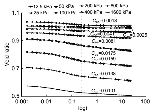
Fig. 8 Void ratio versus time for each load increment on Shanghai clay ( 0^\circ specimen)
