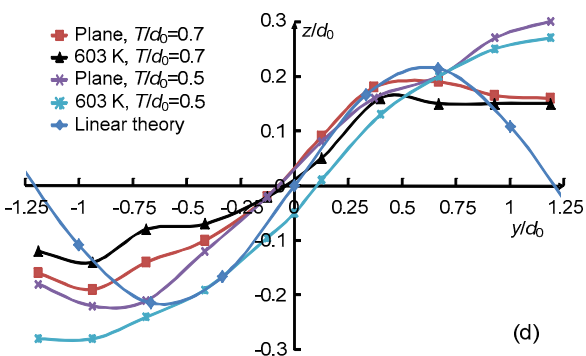
Fig. 9 Bed crosswise morphology, experimental, and theoretical results
