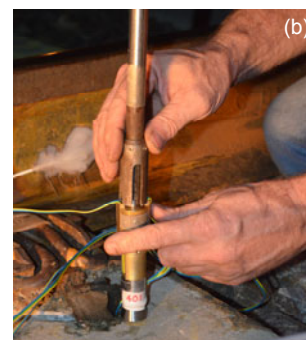
Fig. 7 Photographs of (a) an assembled MDD module along with the LVDT and inner core and (b) MDD module mounted in the insertion tool ready for installation into the drilled hole
