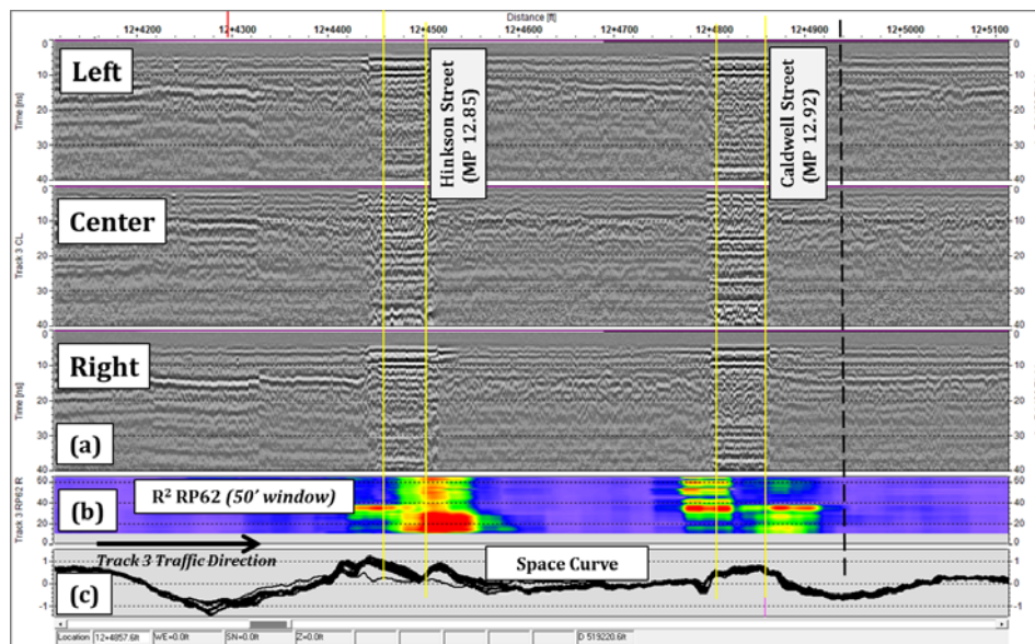
Fig. 3 GPR scans (a), MCO data (b) and space curve (c) for Track 3 at Caldwell street bridge approach (MDD positions: 24.4 m from South abutment)
