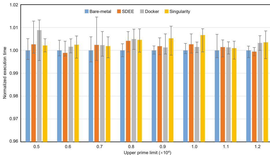
Fig. 9 Overhead of running the SysBench CPU test
