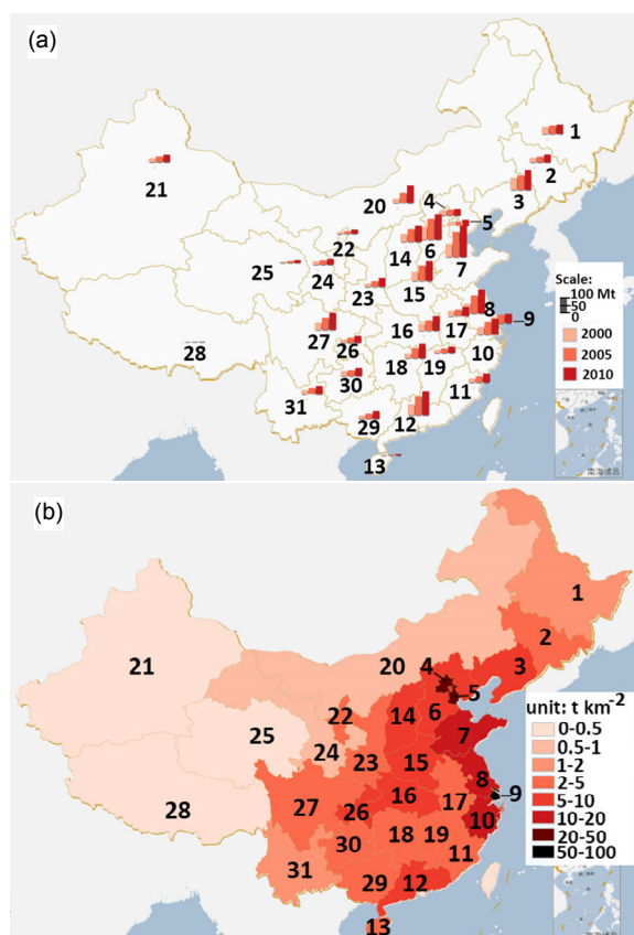
Fig. 5 \text{NO}_x emission trends (a) and distributions (b) of different provinces in China
