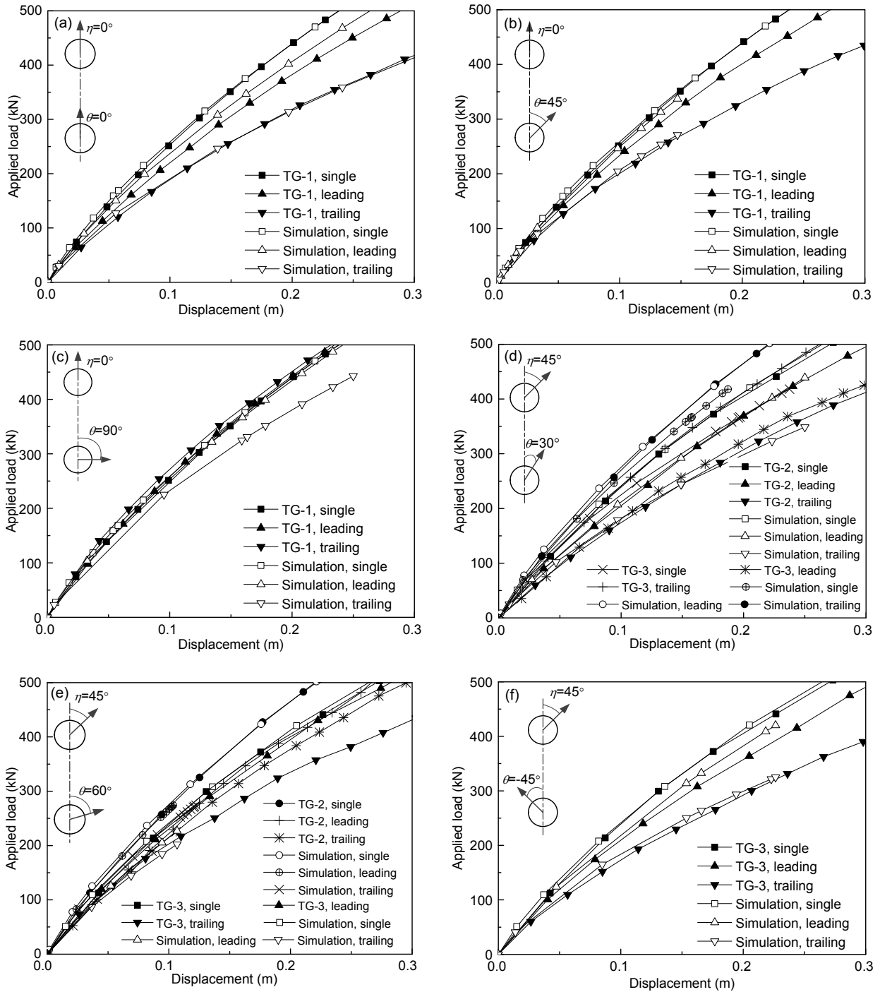
Fig. 5 Applied load-displacement curves
