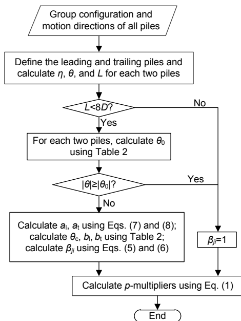
Fig. 11 Flow chart of p -multiplier calculation model
