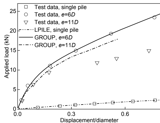
Fig. 13 3×3 pile group subjected to eccentric lateral loading (Kong et al., 2015)
