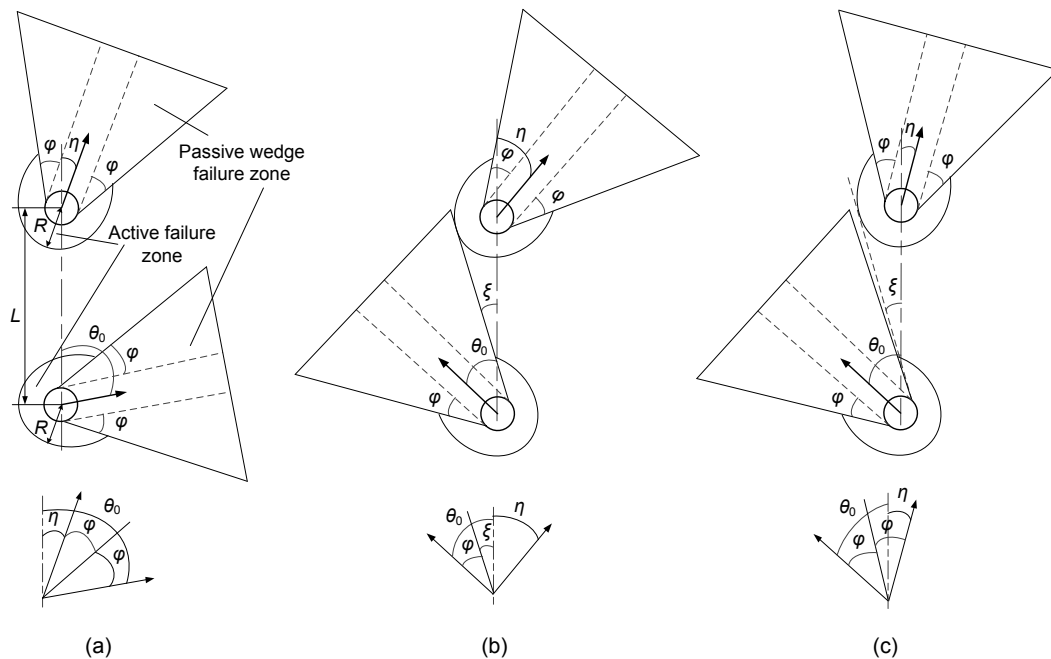
Fig. 7 The critical conditions of two piles with different motion directions (a) 90^\circ - 2\varphi \geq \eta \geq 0^\circ and \theta \geq 0^\circ ; (b) \eta \geq \varphi - \xi and \theta < 0^\circ ; (c) \varphi - \xi > \eta and \theta < 0^\circ
