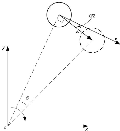
Fig. 1 Motion of a pile rotating around an instantaneous center
