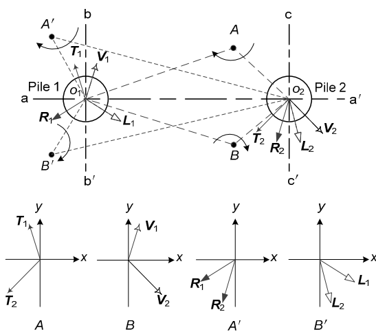
Fig. 2 Motion directions of two piles
