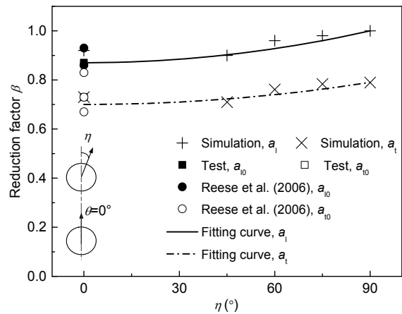
Fig. 9 Relationship between a and \eta at 3D pile spacing
