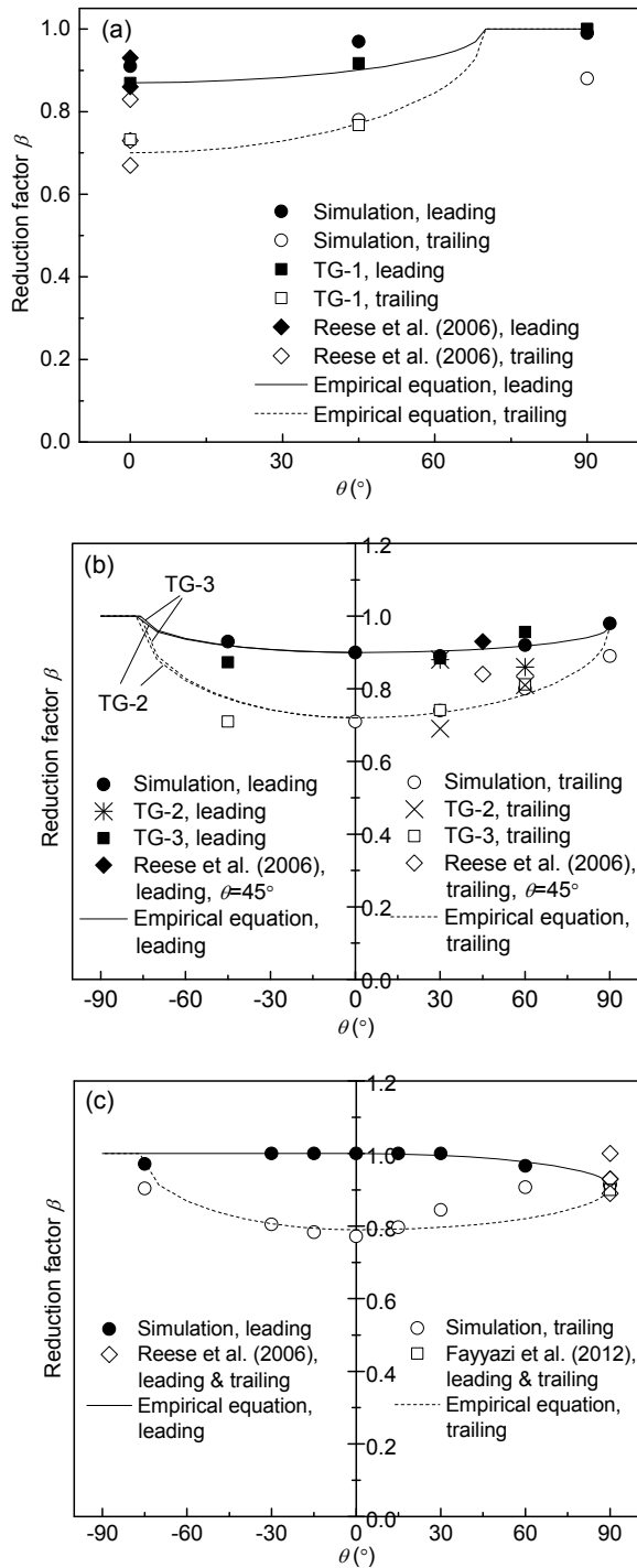
Fig. 6 \beta - \theta curves (a) \eta=0^\circ ; (b) \eta=45^\circ ; (c) \eta=90^\circ
