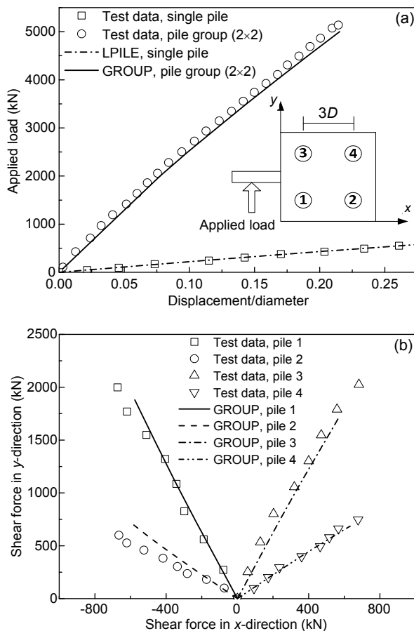
Fig. 12 2×2 pile group subjected to eccentric lateral loading (Gu, 2014)
