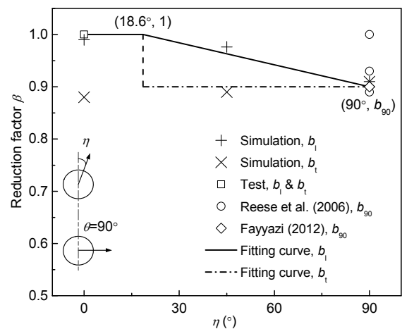
Fig. 10 Relationship between b and \eta at 3D pile spacing ( \theta > 0^\circ )
