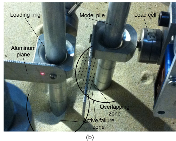
Fig. 4 Layout of the test system (a) Configuration of TG-3; (b) Overlapping of the failure zones ( \eta=45^\circ and \theta=-45^\circ )
